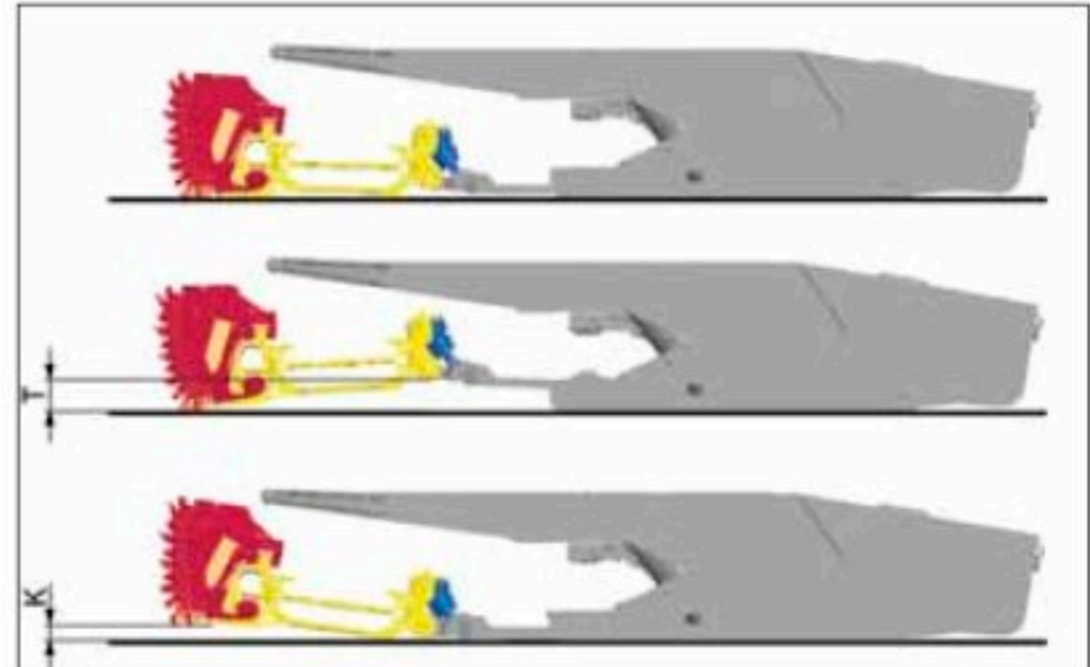
Plow horizon control with outrigger steering system
