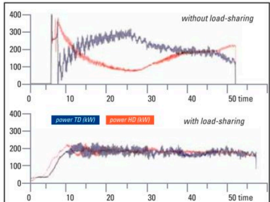
TD = tail drive HD = head drive
