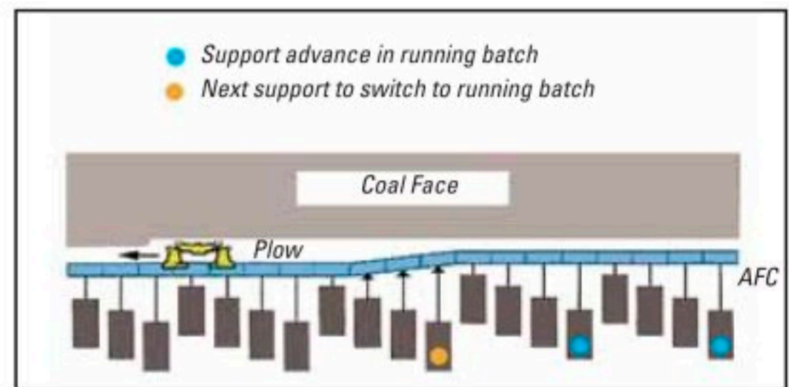
Principle of the incremental plowing method
